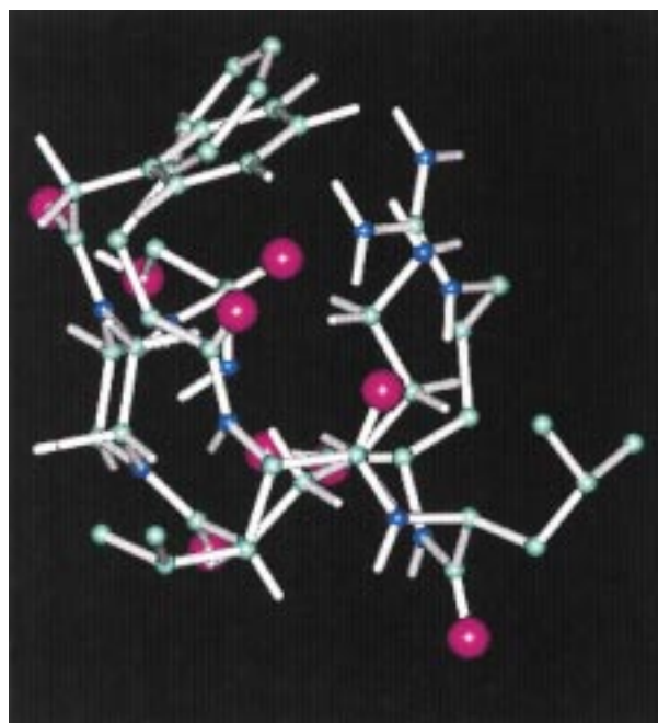
Figure 6. Superimposition of the synthetic analogue 9 with SFLLR using body fit to target method.
