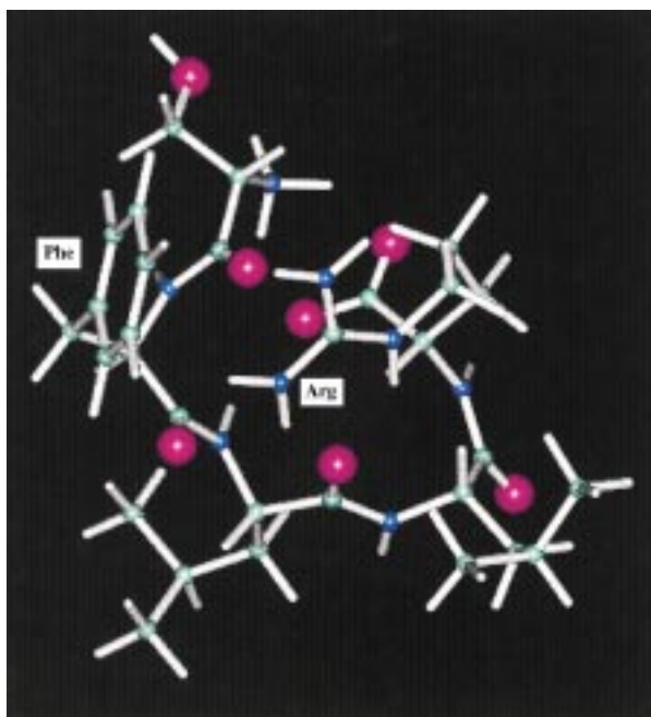
Figure 5. Proposed model of SFLLR generated by imposing distance geometry constraints between Phe and Arg aminoacids and use of molecular dynamics.
