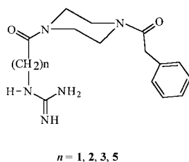
Scheme 1. Nonpeptide TRAP derived mimetics incorporating piperazine.
