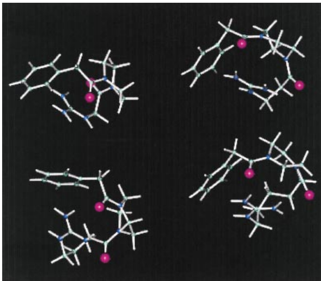
Figure 8. Low energy conformers generated by imposing distance geometry constraints between Phe and Arg aminoacids of synthetic compounds 10 (top, left) 11 (top, right), 12 (bottom, left), and 13 (bottom, right).
