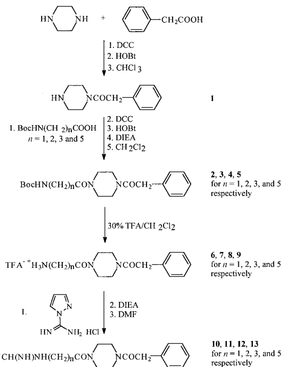
Scheme 2. Synthetic procedure for 1,4-disubstituted piperazine derivatives.
